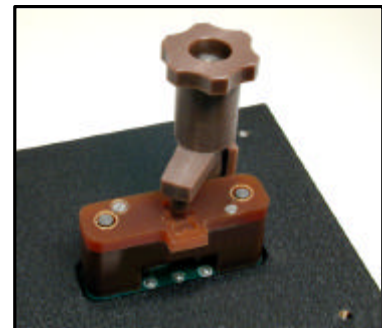
SMD Fixture
